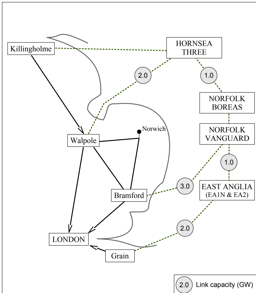
Figure 2: Offshore transmission
